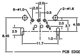
P.C. Board Layout (Top View)
